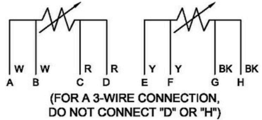
DUAL 4-WIRE WIRING DIAGRAM
